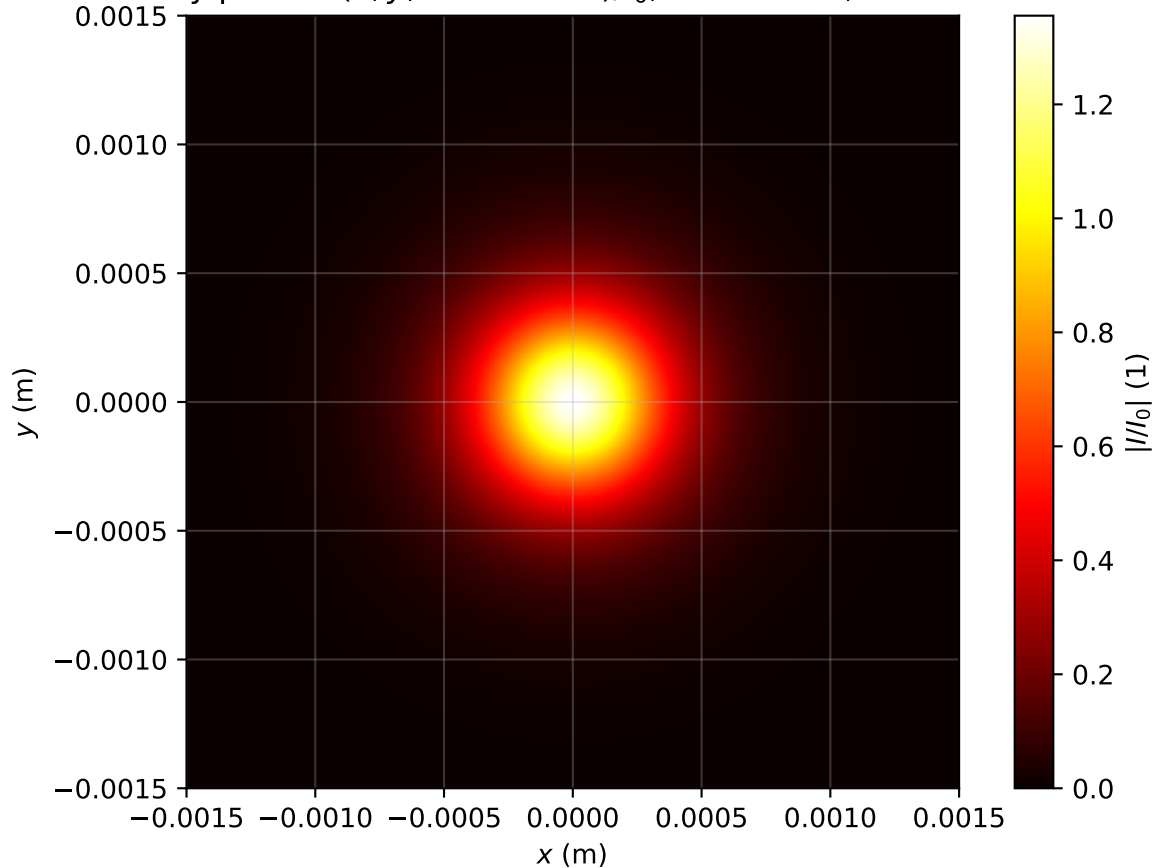
Intensity profile I(x, y, z = 1.433m)/I_0 , P_{in}=0.8P_{cr} , artificial time
